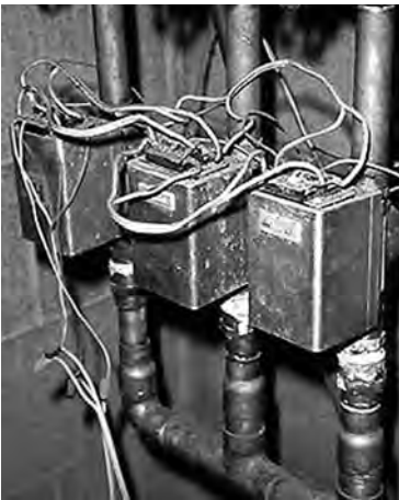
Zone valves: Separate thermostats control each zone valve. Zone valves have switches that activate the burner.
